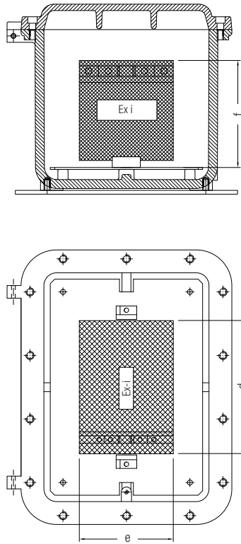
Maximum dimensions of 'Ex ia' equipment that can be installed inside enclosures.
